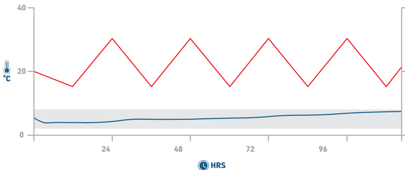
CoolPall™ Flex Water Half Height Single Pod Double Layer EURO +2°C to +8°C Peli BioThermal Summer 101 hours
